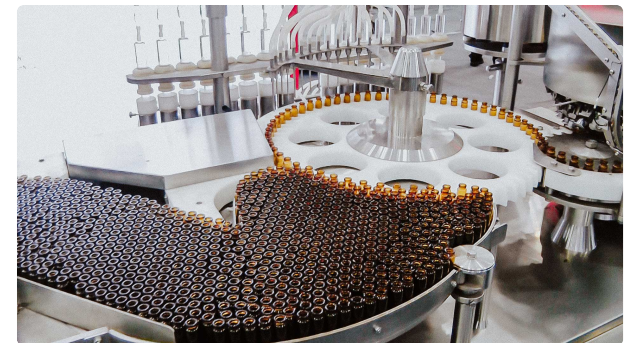
High speed machine for bottling and capping penicillin bottle of aluminum cap
