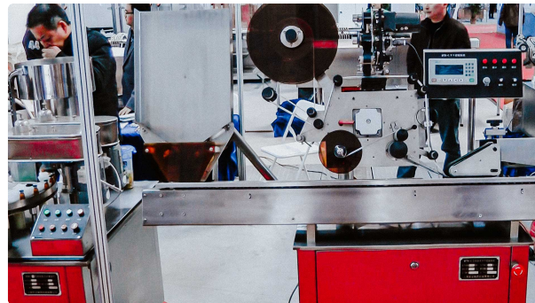
Equipment for self-adhesive labels on glass ampoules
