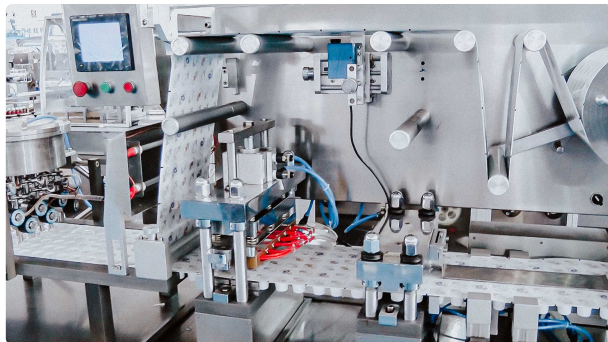
Automatic blister equipment for dispensing and packing disposable cream into blisters
