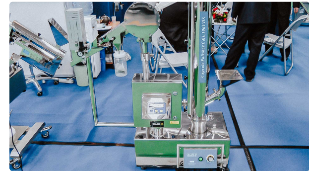
Equipment for cleaning solid gelatin capsules polishing and dust removal
