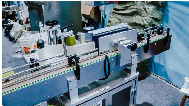
Automatic labeling machine for sticking self-adhesive labels on glass bottles
