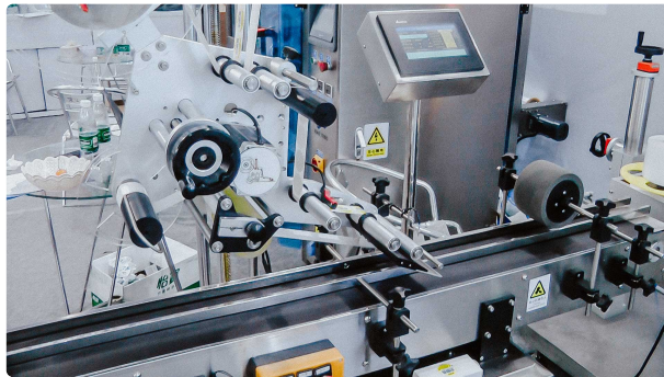
Labeling machine for sticking self-adhesive labels on top of caps and boxes
