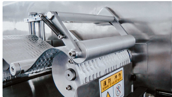
Automatic blister packaging machine for tablets and gelatin capsules in blisters
