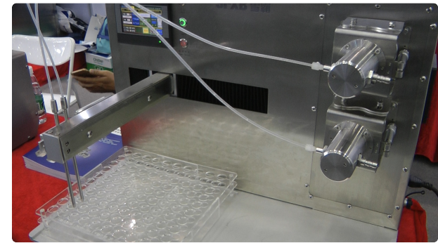
Robot for filling penicillin bottles with liquid in a cassette
