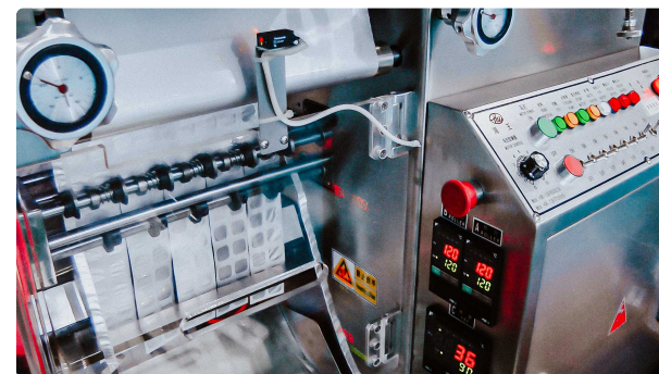
Automatic packaging machine for group packaging of tablets in soft cell packaging
