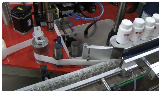
Automatic labeling equipment on penicillin vials in pharmaceutical production
